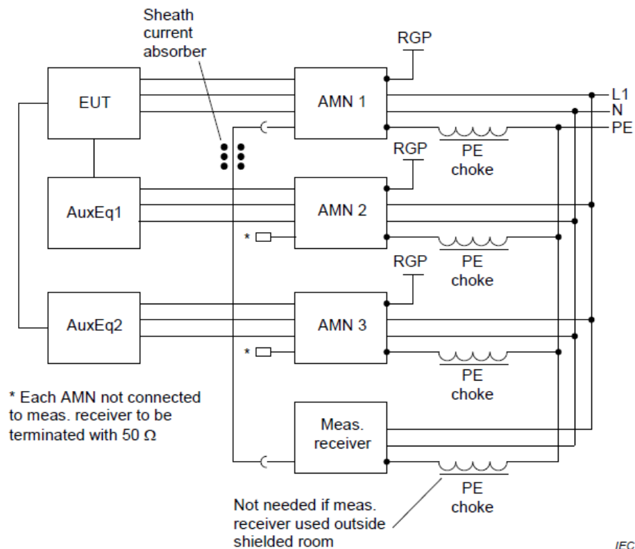
Fig. 4 Arrangement of PE chokes to avoid grounding loops
