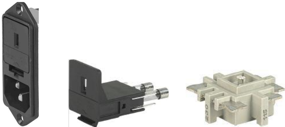
Fig. 6 Low-temperature socket, fuse holder and line voltage selector
